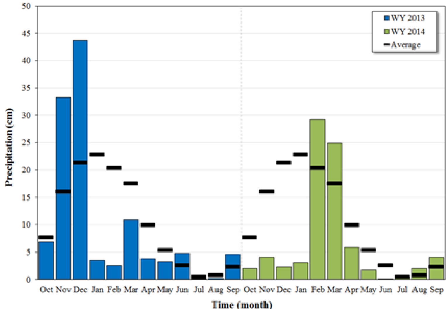
Figure 4. Northern Sierra Monthly Precipitation
