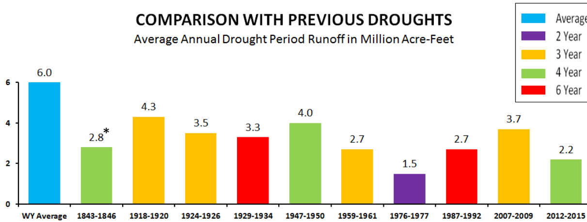
Figure 1. Multiyear droughts of the Sacramento and San Joaquin
