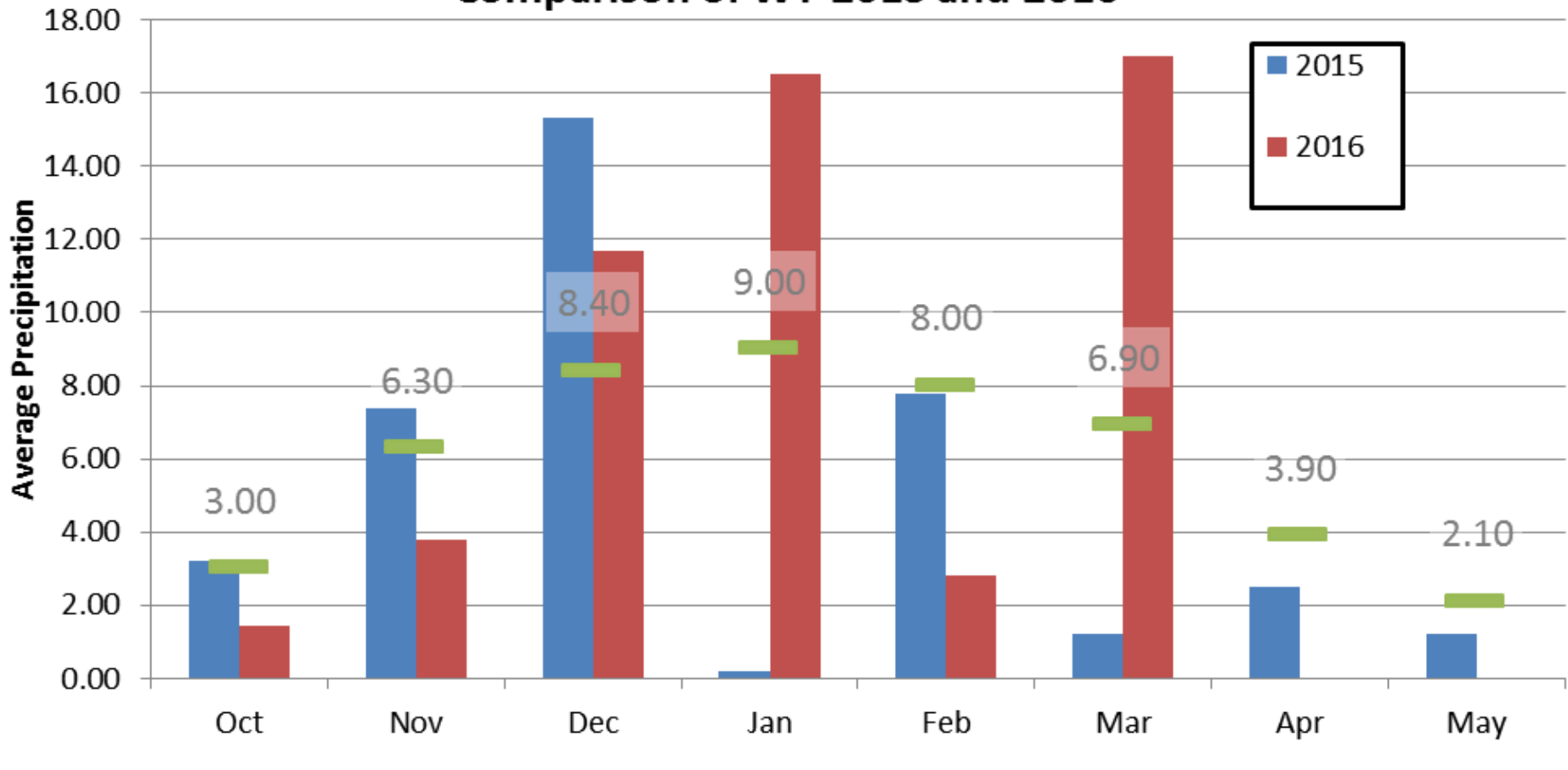
Figure 8. Northern Sierra Precipitation Comparison of WY 2015 and 2016
