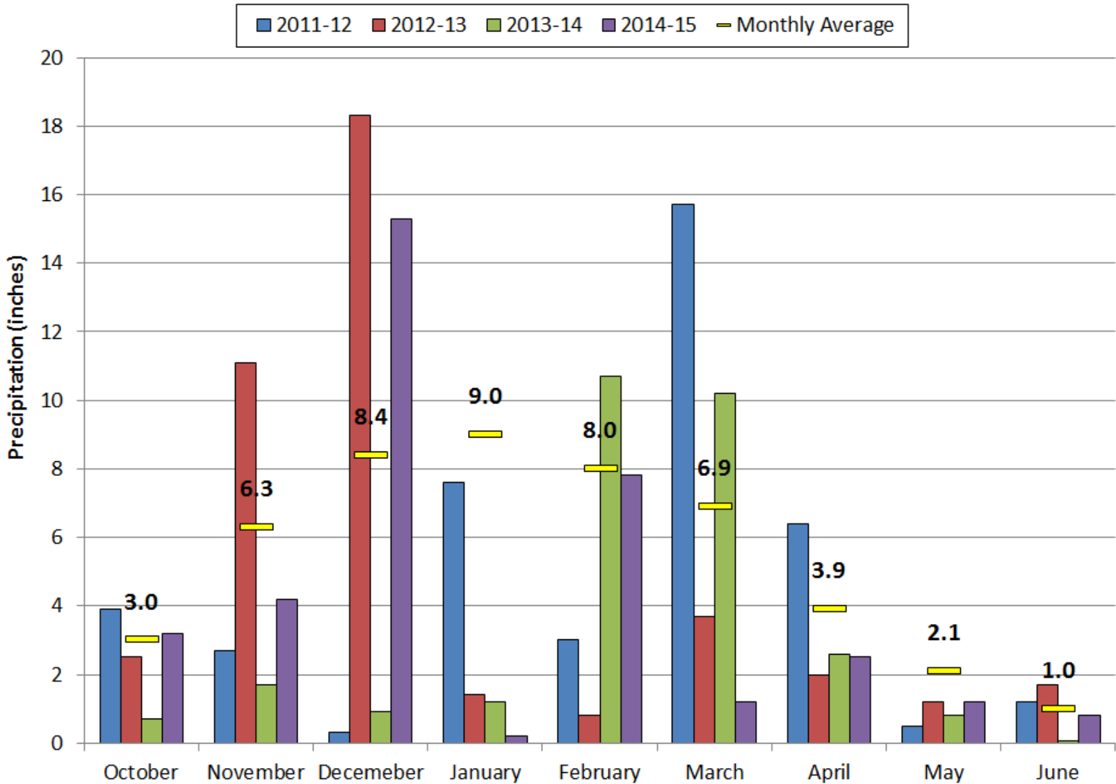
Figure 3. Northern Sierra 8 Station Monthly Precipitation
