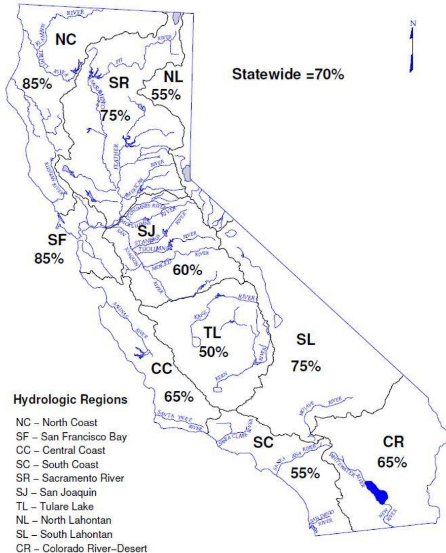
Figure 2. California Precipitation for the 2014-15 Rainy Season.
